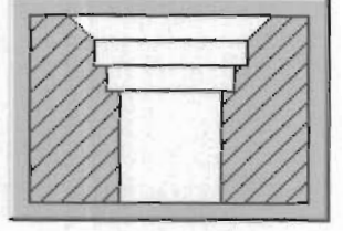
Drilled hole with double counterbore & chamfer Page 15
