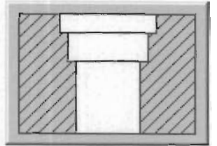
Drilled hole with double counterbore Page 13
